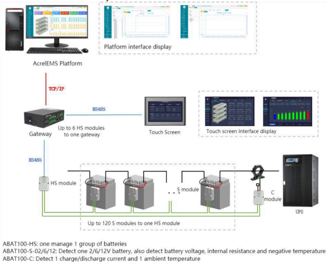
Fig.3 Network plan 2
